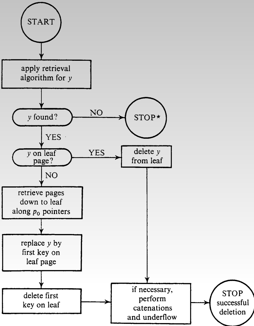
Fig. 6. Deletion algorithm
