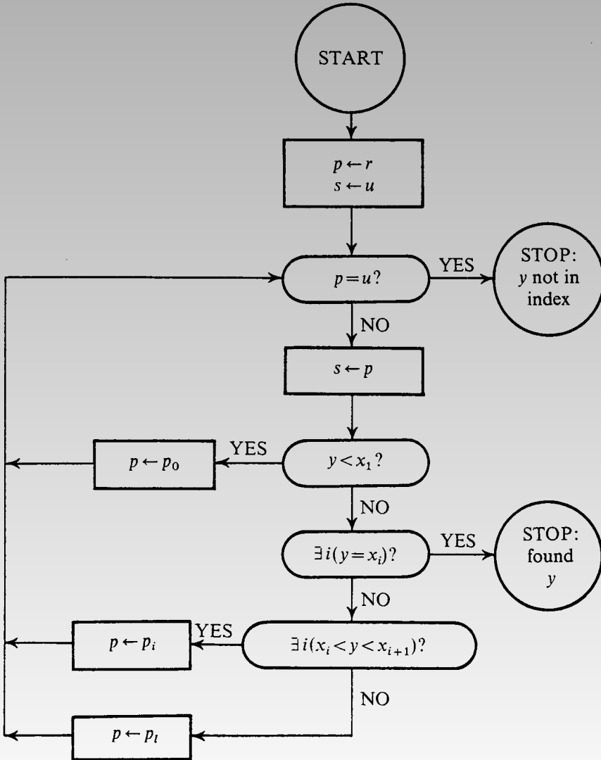
Fig. 3. Retrieval algorithm
