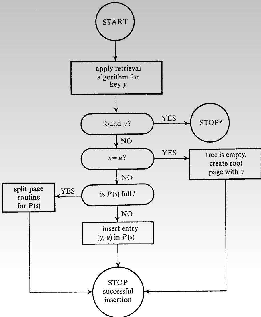
Fig. 4. Insertion algorithm
